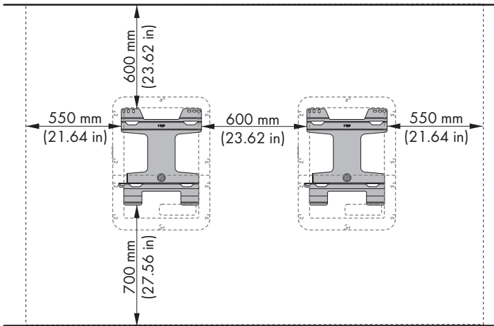
Figure 4 : Recommended clearances(Dimensions in mm (in))
