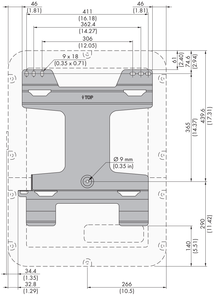
Figure 3 : Position of the anchoring points(Dimensions in mm (in))
