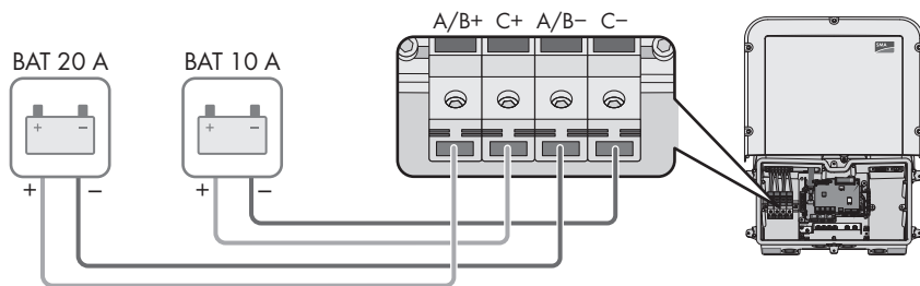
Figure 9 : Connection options (example)
