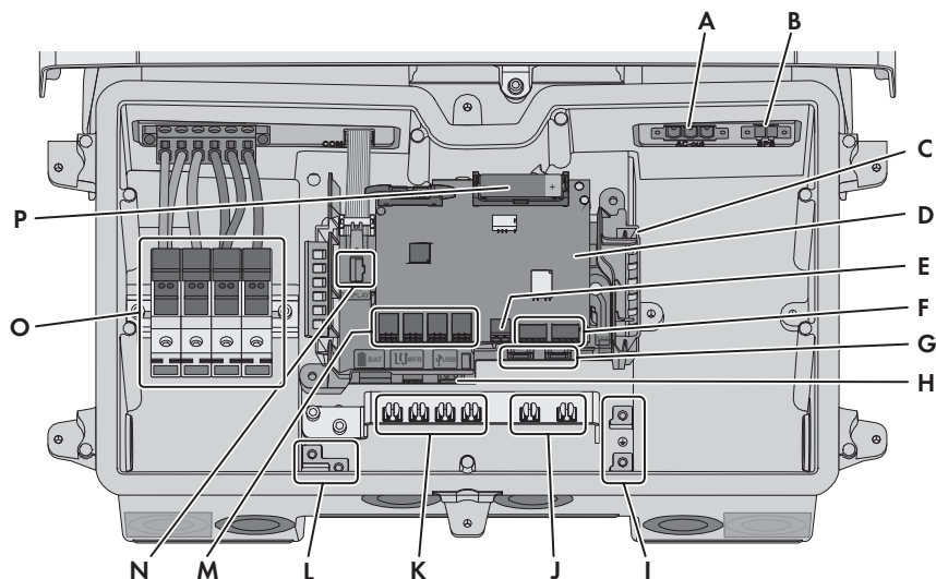
Figure 8 : Connection areas in the interior of the inverter
